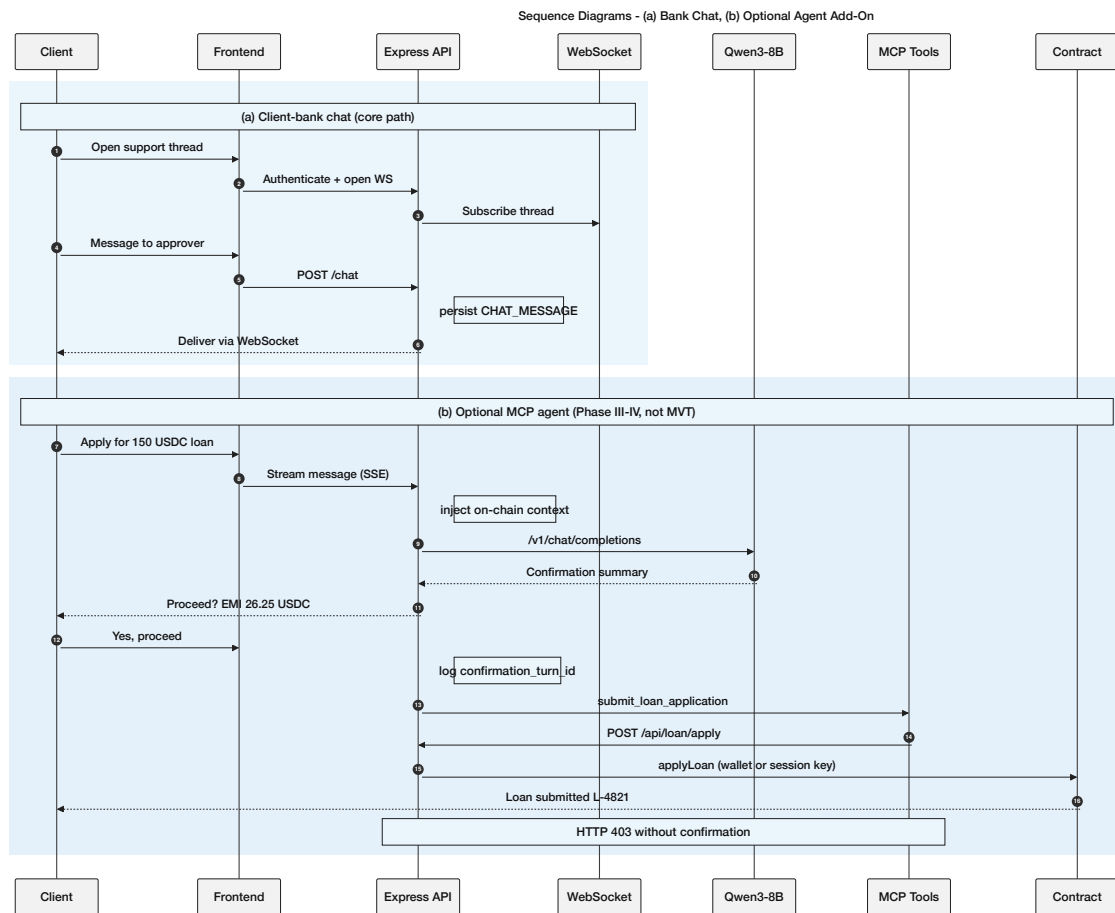
Figure 3.28: Sequence diagrams: (a) client–bank chat over an authenticated WebSocket, and (b) optional MCP agent pipeline (on-chain context injection, read/write routing, human confirmation gate, EIP-7702 session-key signing; Phase III–IV add-on).
