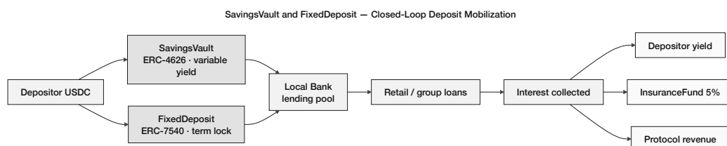
Figure 3.16: SavingsVault (ERC-4626) and FixedDeposit (ERC-7540) mobilize depositor USDC into the Local Bank lending pool; loan interest is split deterministically among depositor yield, the InsuranceFund, and protocol revenue.
