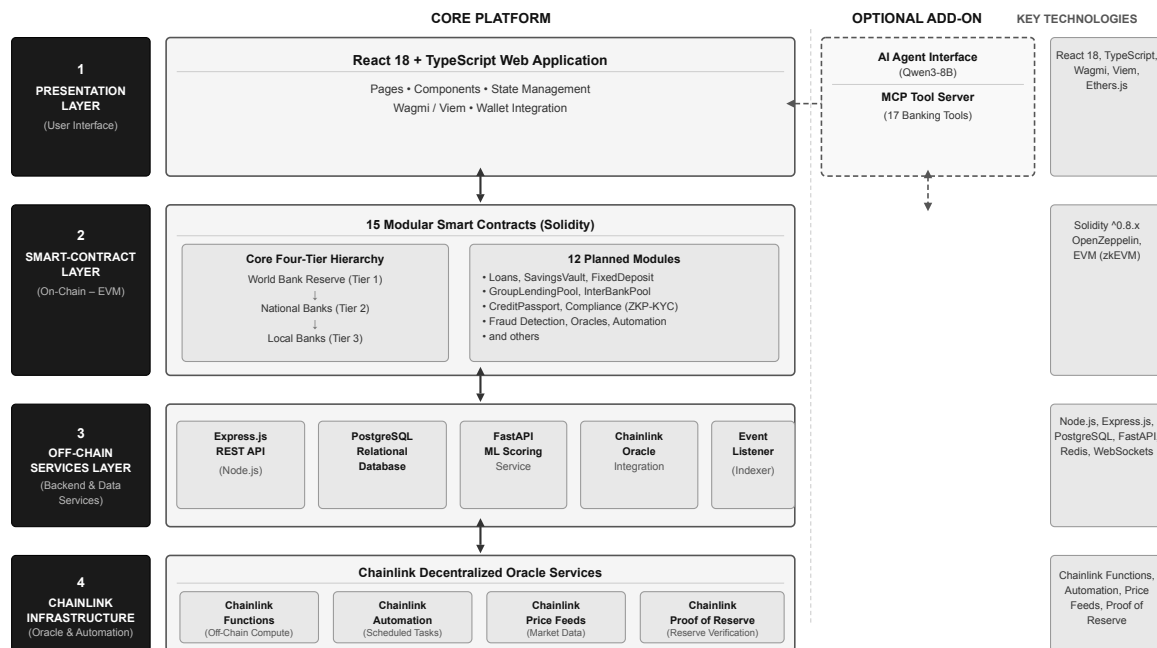
Figure 3.1: Four-layer decentralised application architecture (blockchain-first): presentation (React 18, TypeScript, Wagmi/Viem); smart-contract layer on the EVM (World Bank Reserve, National Bank, Local Bank + twelve planned modules); off-chain services (Express REST API, PostgreSQL, FastAPI ML service, Chainlink oracle integration, event listener, Redis cache); Chainlink infrastructure (Functions, Automation, Price Feeds, Proof of Reserve). Optional add-on: AI agent (Qwen3-8B + MCP) interfaces through the same APIs without altering on-chain logic.
