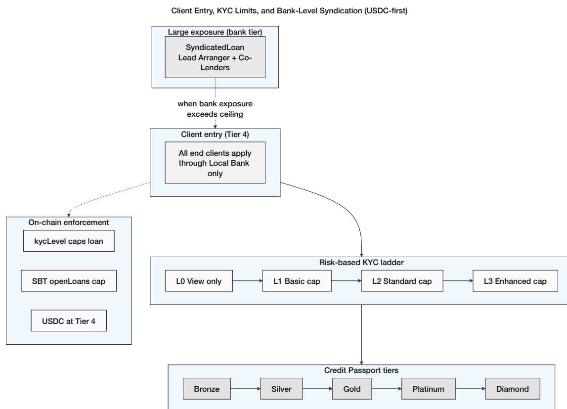
Figure 3.11: Client limits and bank-level syndication. Maximum loan amount is enforced on-chain via kycLevel[wallet] and Credit Passport tier (Sections 3.8.2, 3.12); stablecoin denomination is enforced at Tier 4 (Section 1.10.3); and the SBT carries the simultaneous-loan cap that the GroupLendingPool reads at every application. End clients enter only through Local Banks; exposures above a bank’s prudent ceiling use SyndicatedLoan (Section 3.14.3), not direct client access to National or World Bank tiers.
