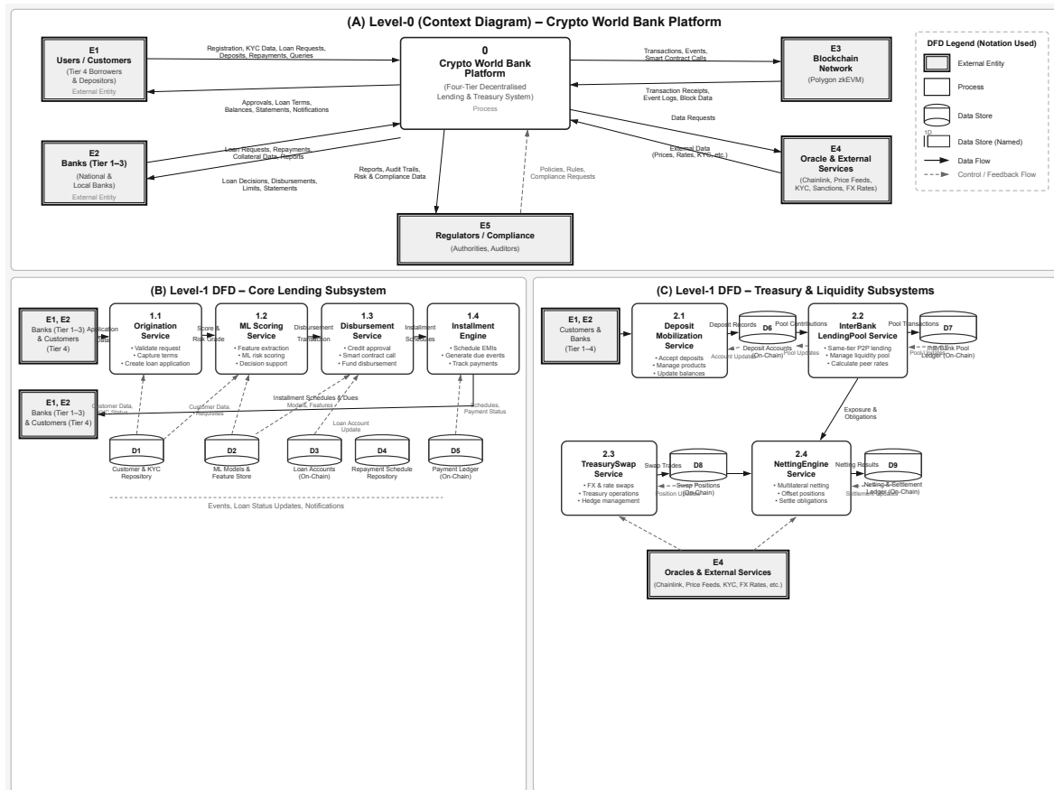
Figure 3.24: Data-flow diagrams: Level-0 context view of the Crypto World Bank platform with five external entities; Level-1 decomposition of the core lending subsystem (origination, ML scoring, disbursement, installment engine, and their data stores); and Level-1 decomposition of the deposit-mobilization, InterBankLendingPool, TreasurySwap, and NettingEngine subsystems.
