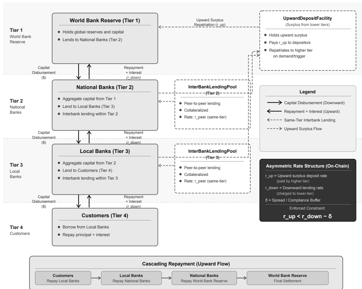
Figure 3.29: Four-tier hierarchical capital flow with cascading repayment, plus the same-tier interbank-lending pools (InterBankLendingPool, Section 3.14.1) and the upward-surplus repatriation facility (UpwardDepositFacility, Section 3.14.2). The asymmetric rate structure ( r_{up} < r_{down} - \delta ) is enforced on-chain.
