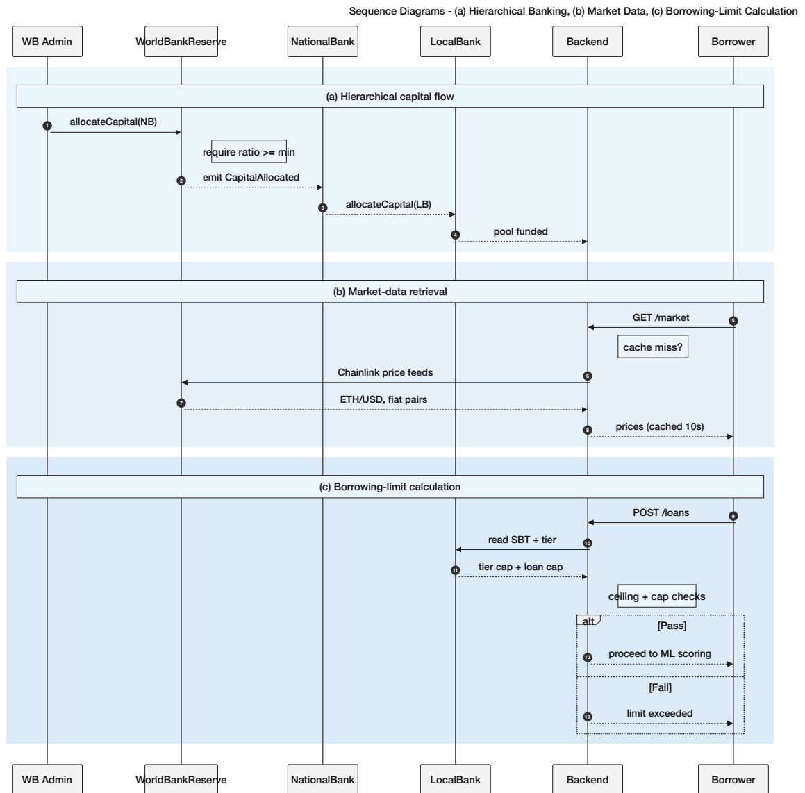
Figure 3.27: Sequence diagrams: (a) hierarchical capital flow with reserve-ratio gates at every tier, (b) market-data retrieval via cached Chainlink feeds, (c) borrowing-limit calculation reading the credit-passport SBT before ML scoring.
