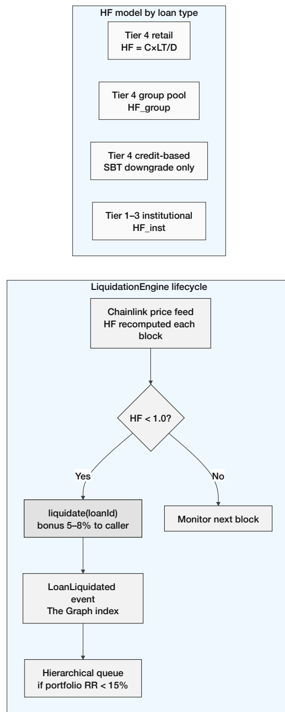
Figure 3.15: LiquidationEngine: tier-specific Health Factor models (retail collateral, group pool, credit-based SBT downgrade, institutional reserve surplus) and the on-chain liquidation lifecycle (Chainlink price update → liquidate() with 5–8% bonus → hierarchical portfolio queue when reserve ratio falls below 15%).
