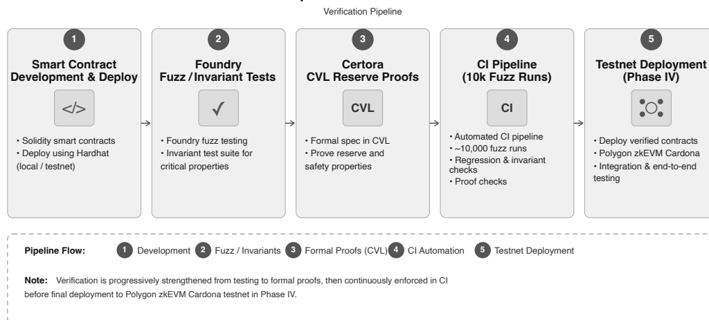
Planned Development and Verification Toolchain
