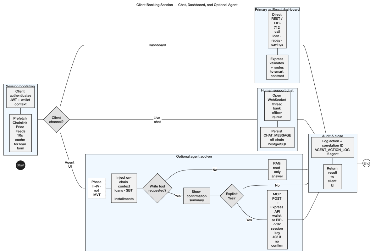
Figure 3.23: Client banking session activity flow: authenticated session bootstrap with Chainlink price prefetch, then channel routing to the primary React dashboard path, human WebSocket chat, or the optional MCP agent add-on (confirmation gate and AGENT_ACTION_LOG audit before session close).
