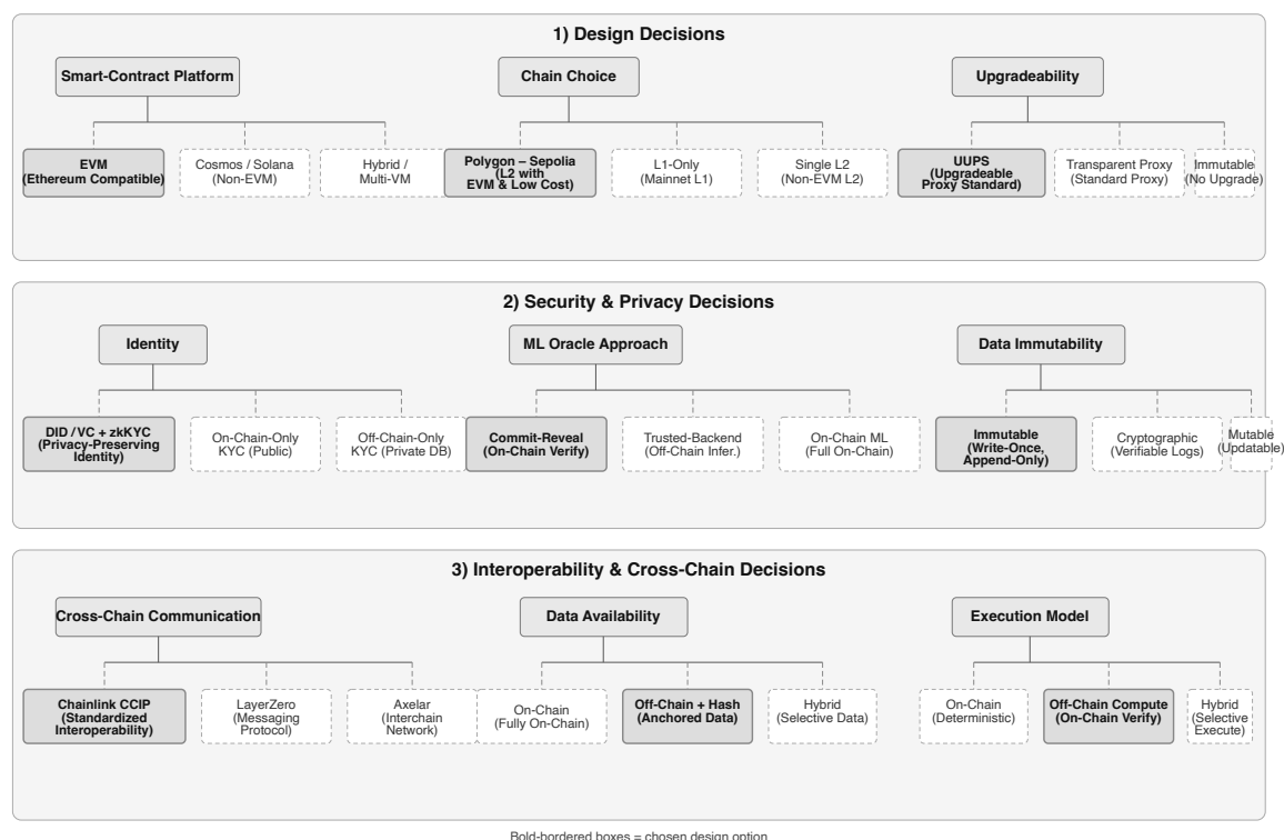
Figure 4.11: Key design decisions and alternatives considered: smart-contract platform (EVM vs. Cosmos / Solana), chain choice (Polygon + Sepolia vs. L1-only vs. single L2), upgradeability (UUPS vs. Transparent Proxy vs. immutable), identity (DID/VC + zkKYC vs. raw on-chain KYC vs. off-chain-only), ML oracle (commit-reveal vs. trusted-backend vs. on-chain ML), and cross-chain bridge (Chainlink CCIP vs. LayerZero vs. Axelar).
