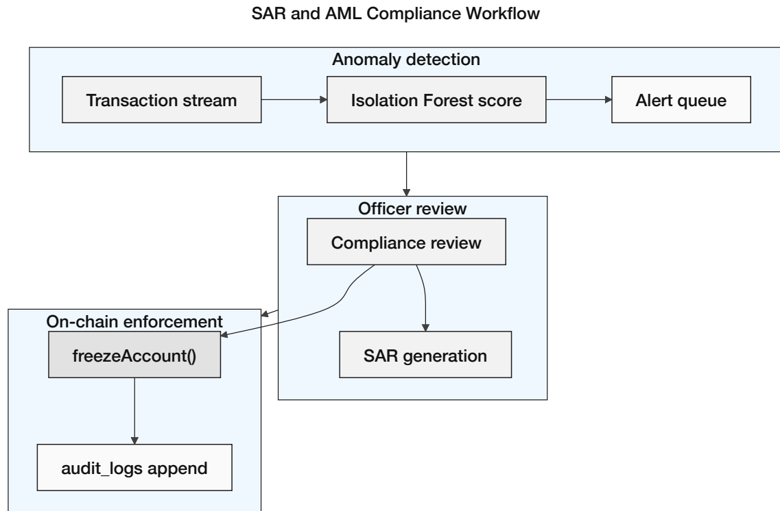
Figure 3.32: SAR and AML compliance workflow: Isolation Forest anomaly detection, compliance officer review queue, optional SAR report generation, on-chain freezeAccount via onlyApprover, and append-only audit_logs record.
