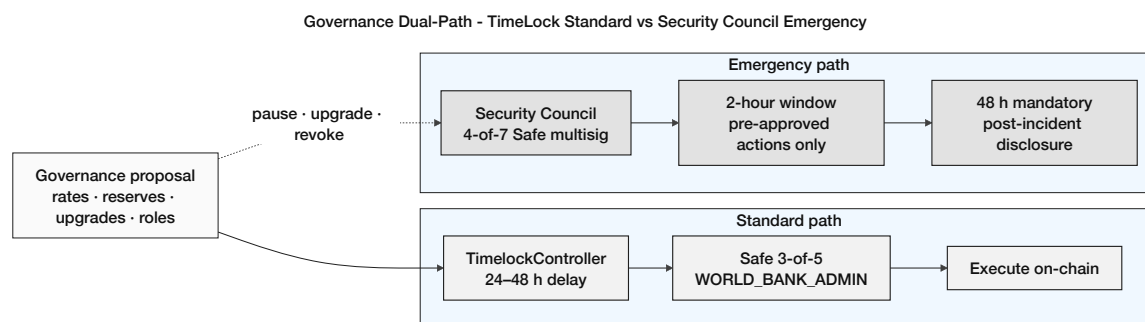
Figure 3.31: Governance dual-path: (a) standard TimeLock-gated parameter changes and upgrades via Safe 3-of-5, and (b) Security Council emergency path (4-of-7) for pre-approved pause, upgrade, and role-revocation actions within a 2-hour window with mandatory 48-hour disclosure.
