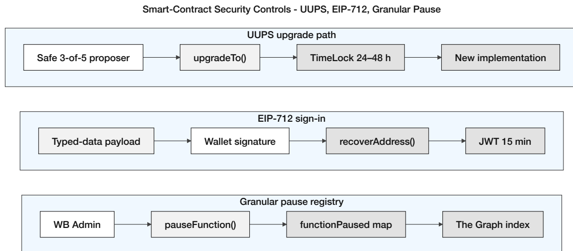
Figure 3.34: Smart-contract security controls: (a) UUPS (ERC-1822) upgrade path with TimeLock-gated authorization; (b) EIP-712 sign-in (typed-data v4 with domain separation and 15-minute JWT); (c) granular per-function pause registry indexed by The Graph for transparent governance.
