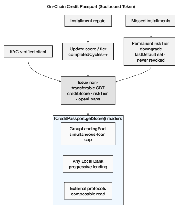
Figure 3.17: Credit Passport SBT lifecycle: non-transferable credential issued after KYC, updated on repayment, permanently downgraded (never revoked) on default, and exposed read-only via ICreditPassport.getScore() to GroupLendingPool, peer Local Banks, and external protocols.
