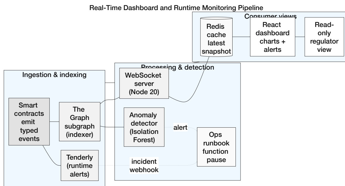
Figure 4.5: Real-time dashboard and runtime monitoring pipeline: smart contracts emit typed events; The Graph indexes them and pushes to a Node WebSocket server which renders the React dashboard via a Redis snapshot. Tenderly runtime alerts and an Isolation-Forest anomaly detector feed the operations runbook with the granular-pause control surface of Section 3.19.
