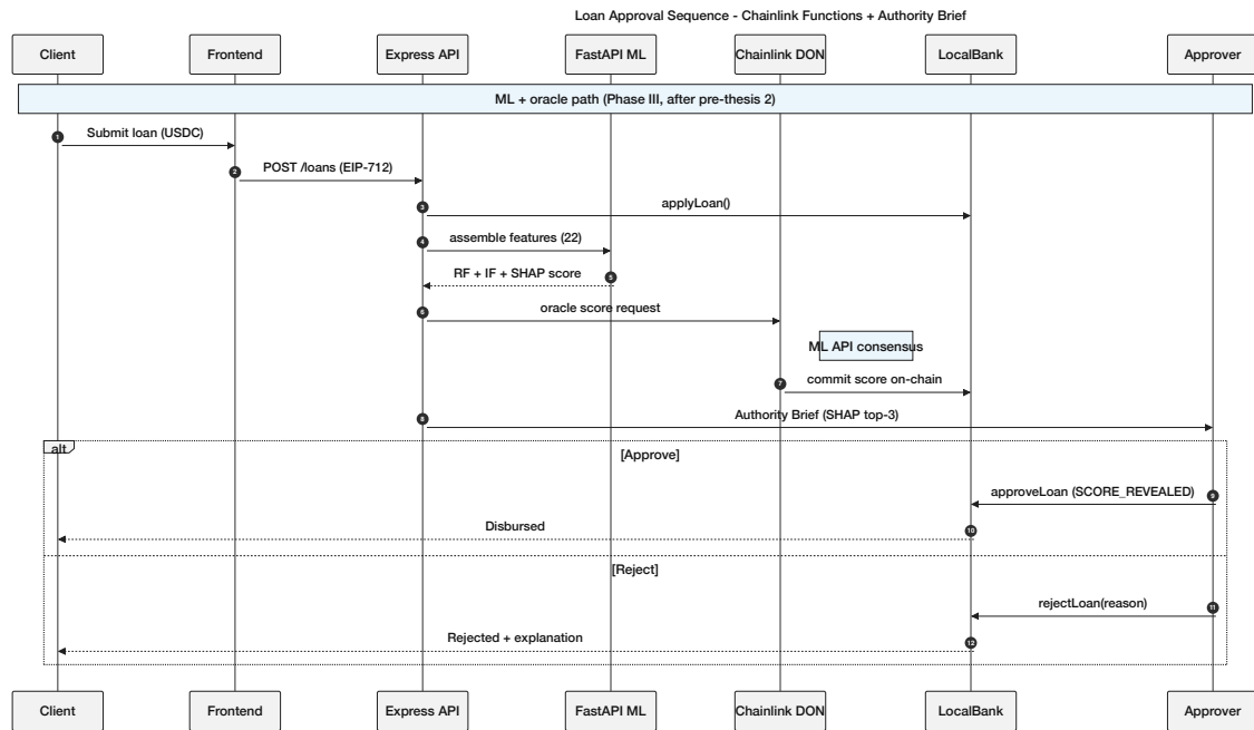
Figure 3.25: Sequence diagram for the loan-approval flow with reject alternative: the client submits an EIP-712 signed request, the ML oracle returns a SHAP-explained score via commit-reveal, and the approver either approves (revealing the commit) or rejects (with reason logged on-chain).
