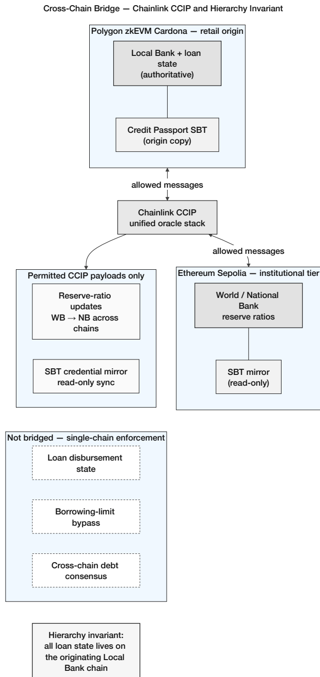
Figure 3.18: Chainlink CCIP cross-chain architecture: Polygon zkEVM Cardona holds authoritative retail loan state; Ethereum Sepolia hosts institutional reserve tiers. CCIP carries only reserve-ratio updates and read-only SBT mirrors—loan state and borrowing-limit enforcement remain on the originating chain.
