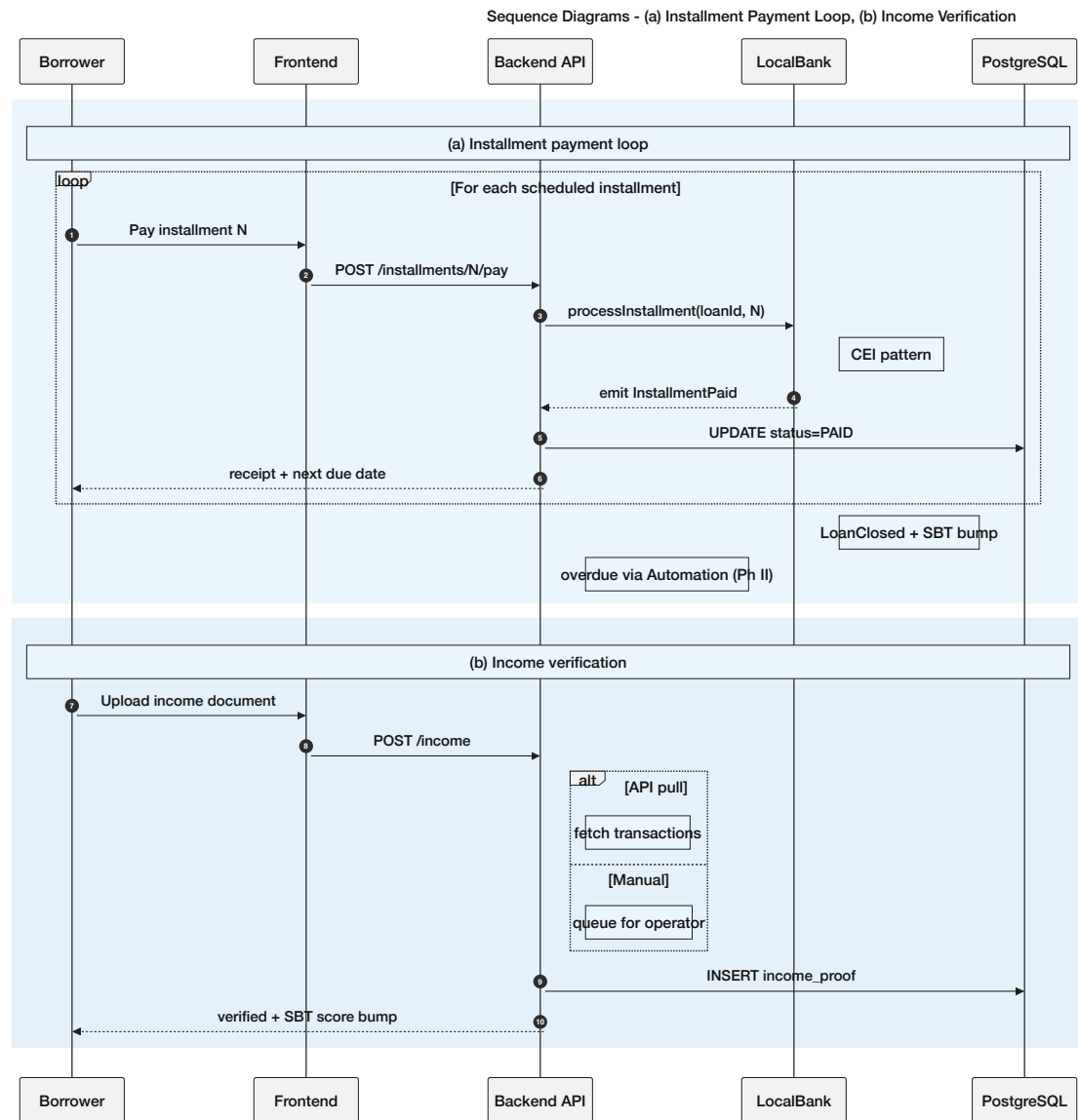
Figure 3.26: Sequence diagrams: (a) installment payment loop using the CEI pattern with SBT update on the final installment, and (b) income verification with Open-Banking pull or manual officer review.
