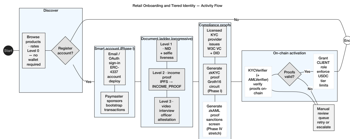
Figure 3.22: Retail onboarding and identity activity flow: progressive ladder from L0 product browse through ERC-4337 smart-account creation, document capture (L1–L3), licensed KYC provider VC issuance, zkKYC/zkAML proof generation, and on-chain CLIENT role activation with tier limits enforced.
